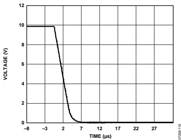
Figure 18. Full-Scale Negative Step
