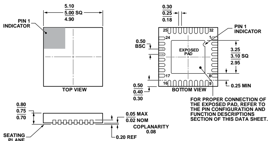
Figure 59. 32-Lead Lead Frame Chip Scale Package [LFCSP_WQ] 5 mm x 5 mm Body, Very Very Thin Quad (CP-32-7) Dimensions shown in millimeters
