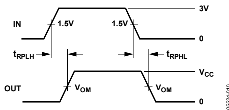
Figure 30. Receiver Propagation Delays
