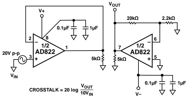
Figure 31. Crosstalk Test Circuit
