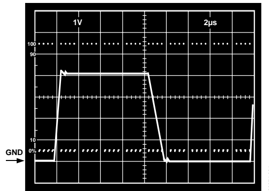
Figure 34. V_S = 5\text{ V} , 0 V; Unity-Gain Follower Response to 0 V to 4 V Step
