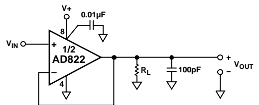
Figure 35. Unity-Gain Follower
