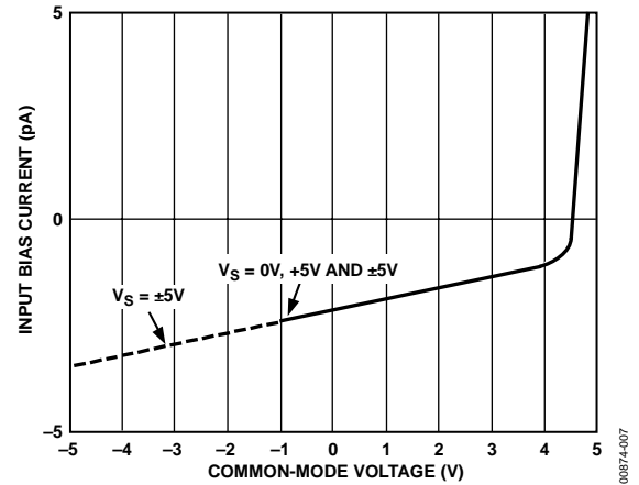
Figure 7. Input Bias Current vs. Common-Mode Voltage; V_S = 5\text{ V}, 0\text{ V}, and V_S = \pm 5\text{ V}
