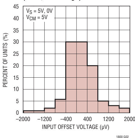
V_{OS} Distribution, V_{CM} = 5\text{V} (SO-8, NPN Stage)
