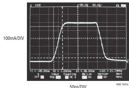
Laser Driver Amplifier 500mA Pulse Response
