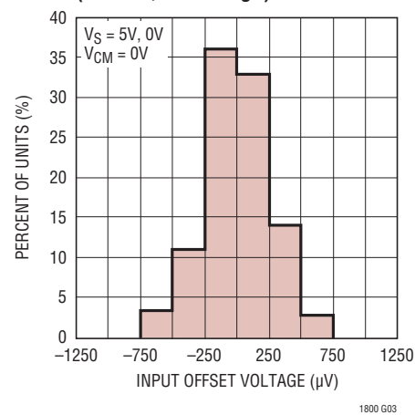
V_{OS} Distribution, V_{CM} = 0\text{V} (SOT-23, PNP Stage)
