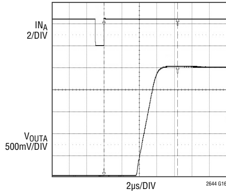
IN X to V OUTX Delay Full-Scale Transition
