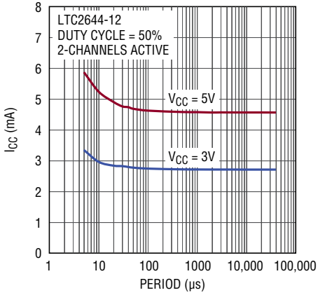
Supply Current vs Input Period ( t_{PER} )
