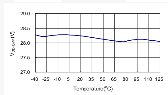
Figure 8. V_{\text{DD}} Over-Voltage Protection Threshold
