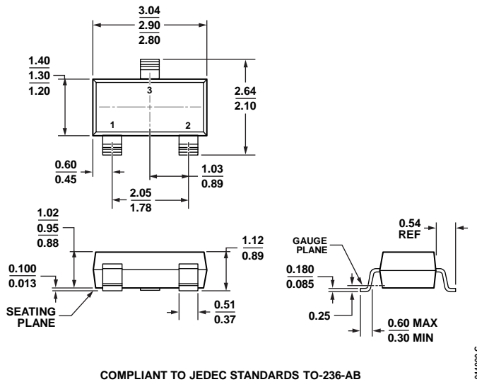
Figure 25. 3-Lead Small Outline Transistor Package [RT-SOT-23-3] (RT-3) Dimensions shown in millimeters
