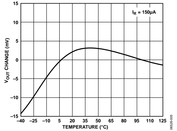
Figure 5. ADR5045 V_{OUT} Change vs. Temperature
