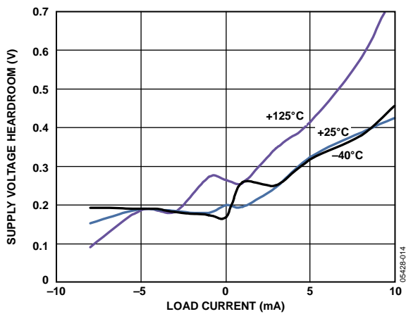
Figure 18. ADR441 Supply Voltage Headroom vs. Load Current
