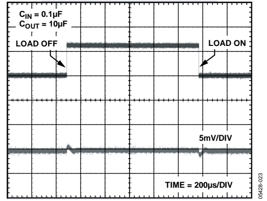
Figure 26. ADR441 Load Transient Response
