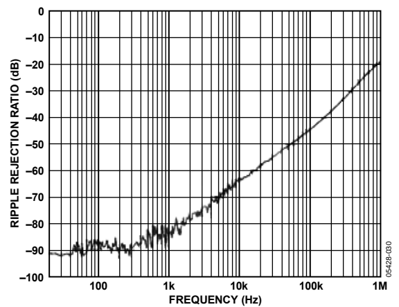
Figure 34. Ripple Rejection Ratio vs. Frequency
