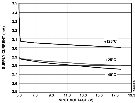
Figure 12. ADR445 Supply Current vs. Input Voltage
