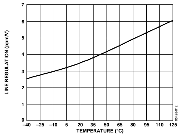
Figure 16. ADR445 Line Regulation vs. Temperature
