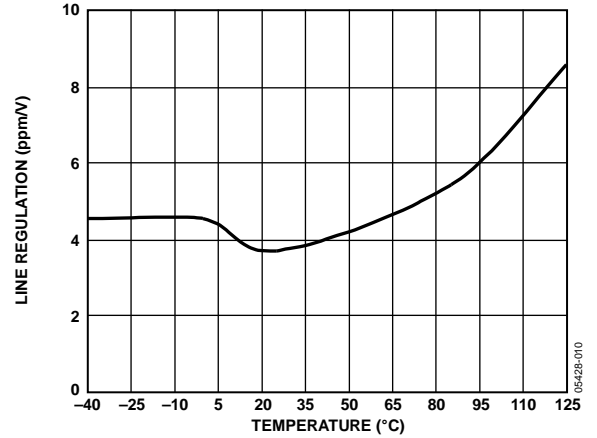
Figure 14. ADR441 Line Regulation vs. Temperature
