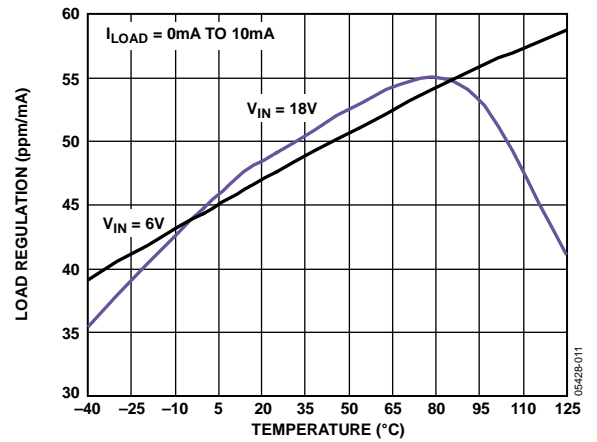
Figure 15. ADR441 Load Regulation vs. Temperature
