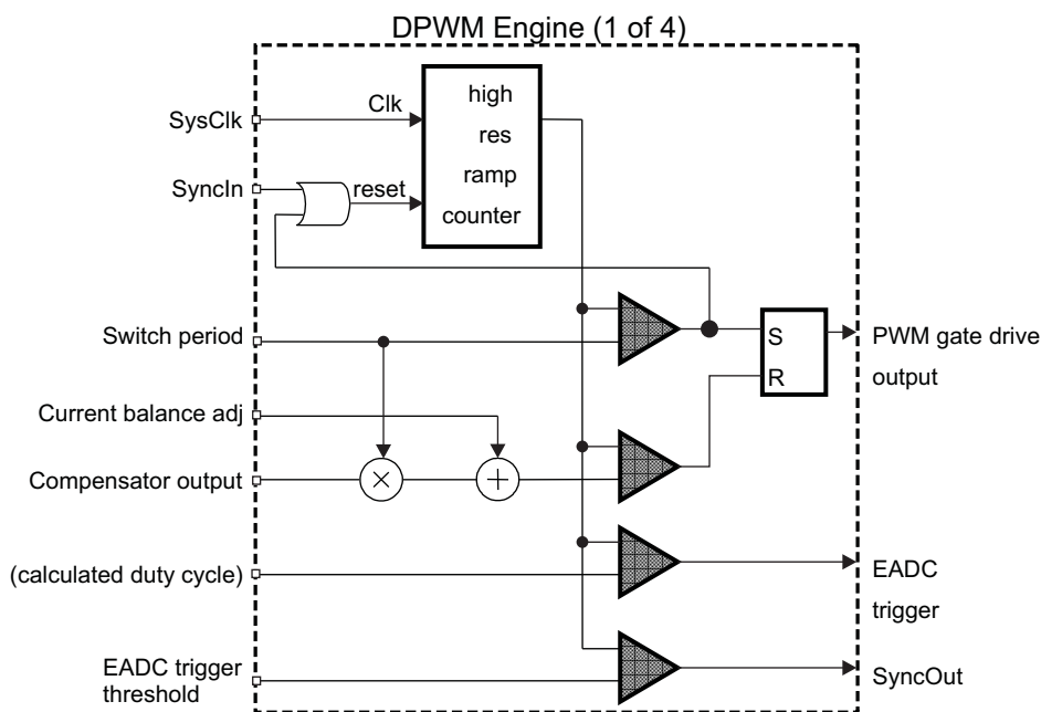
Figure 10. DPWM Engine
