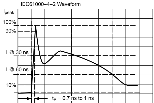
Figure 10. IEC61000-4-2 Spec
