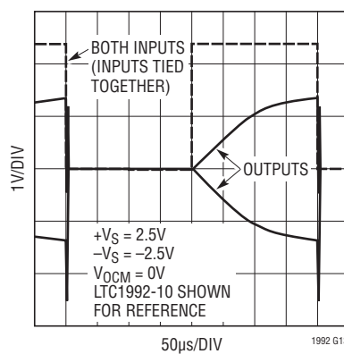
Input Common Mode Overdrive Recovery (Expanded View)
