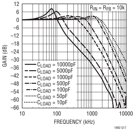
Differential Input Differential Gain vs Frequency, V_S = \pm 2.5V
