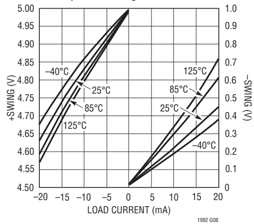
Output Voltage Swing vs Output Load, VS = 5V
