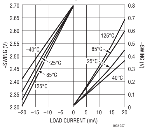
Output Voltage Swing vs Output Load, VS = 2.7V
