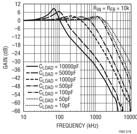
Single-Ended Input Differential Gain vs Frequency, V_S = \pm 2.5V
