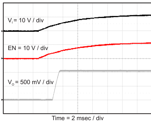
Figure 29. TPS562209 Start Up Relative to V_i
