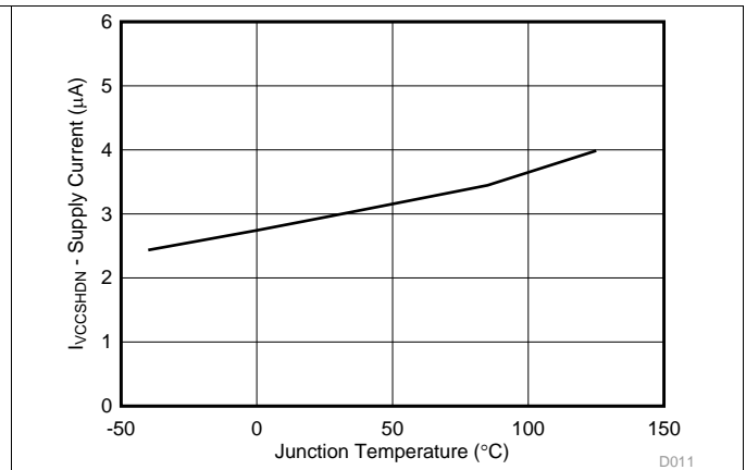
Figure 11. VIN Shutdown Current vs Junction Temperature
