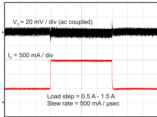
Figure 28. TPS562209 Transient Response
