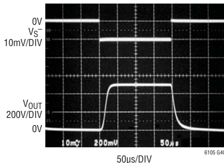
Step Response V_{SENSE} = 0V to 10mV , C_L = 1000pF , V_S^+ = 0V
