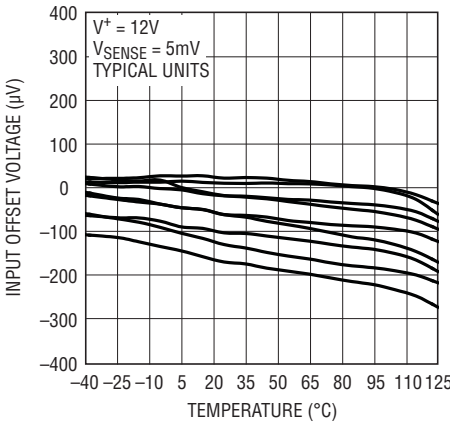
Input Offset Voltage vs Temperature, V_S^+ = 12\text{V}
