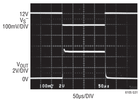
Step Response V_{SENSE} = 0V to 100mV , R_{IN} = 100\Omega
