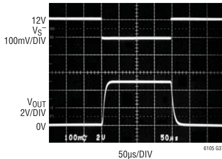
Step Response V_{SENSE} = 0V to 100mV , C_L = 1000pF , V_S^+ = 12V
