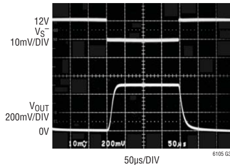
Step Response V_{SENSE} = 0V to 10mV , C_L = 1000pF , V_S^+ = 12V
