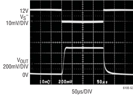
Step Response V_{SENSE} = 0V to 10mV , V_S^+ = 12V
