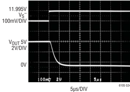
Step Response V_{SENSE} = 100mV to 5mV
