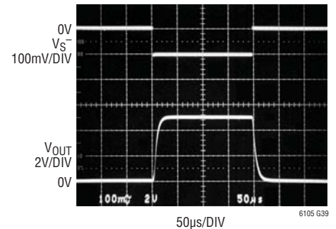
Step Response V_{SENSE} = 0V to 100mV , C_L = 1000pF , V_S^+ = 0V
