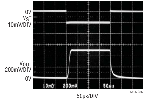
Step Response V_{SENSE} = 0V to 10mV , V_S^+ = 0V
