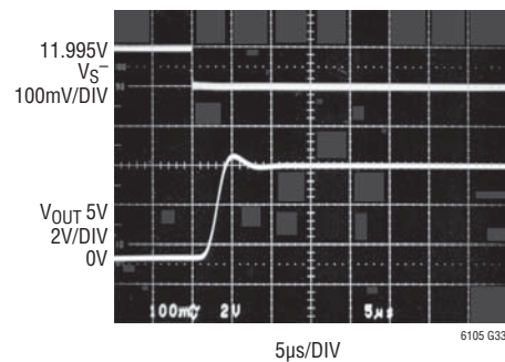
Step Response V_{SENSE} = 5mV to 100mV
