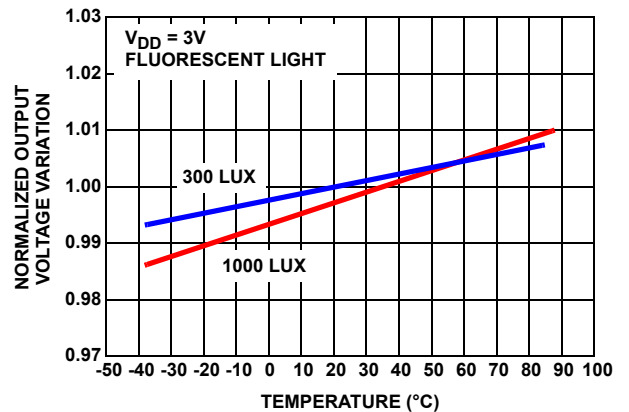
FIGURE 12. NORMALIZED OUTPUT VOLTAGE vs TEMPERATURE
