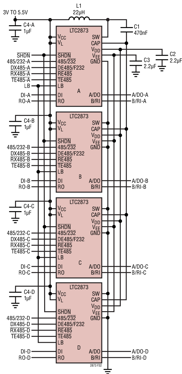
Figure 32. Quad Transceiver
