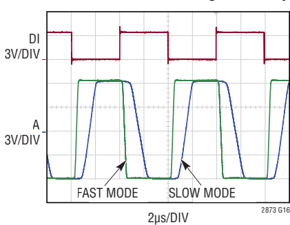
RS232 Driver Switching at 250kbps
