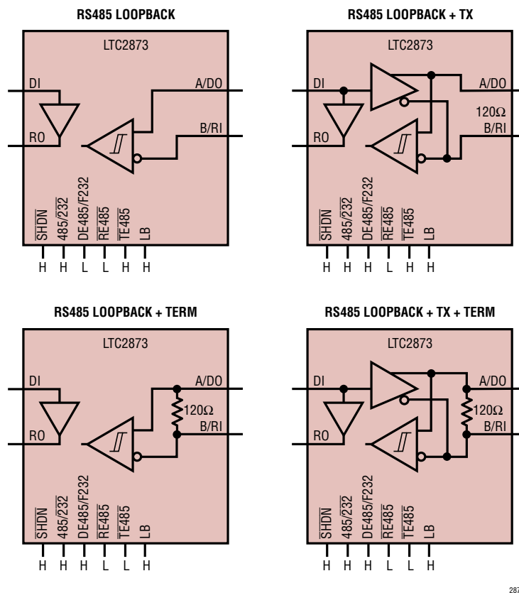
Figure 26. RS485 + Loopback Configurations
