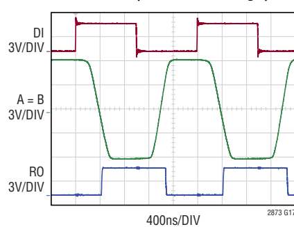
RS232 Operation at 1Mbps FAST Mode (DE485/F232 High)
