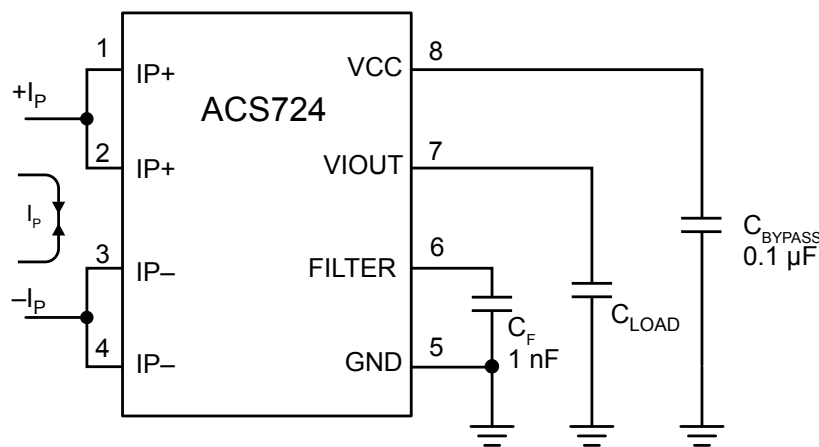
Typical Application
