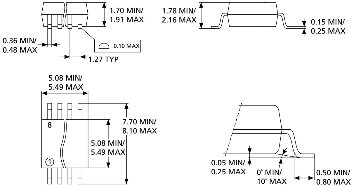
Figure 36: S08W 208 mils Body Width
