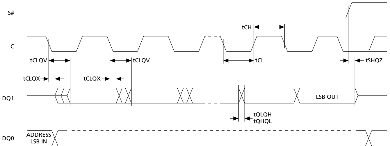
Figure 33: Output Timing
