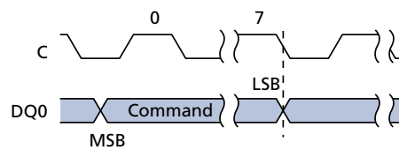
Figure 25: BULK ERASE Command Sequence
