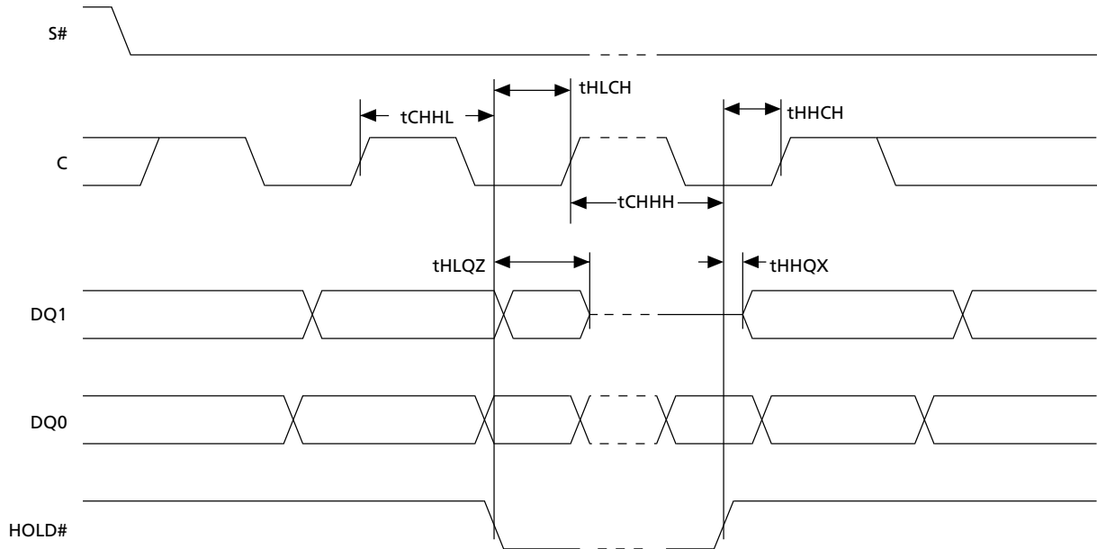
Figure 32: Hold Timing
