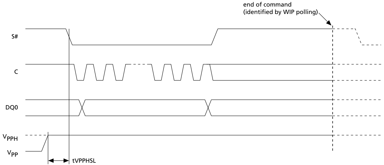
Figure 34: VPPH Timing
