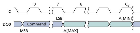
Figure 23: SUBSECTOR ERASE Command Sequence
