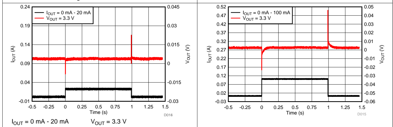
Figure 15. Load Transient
