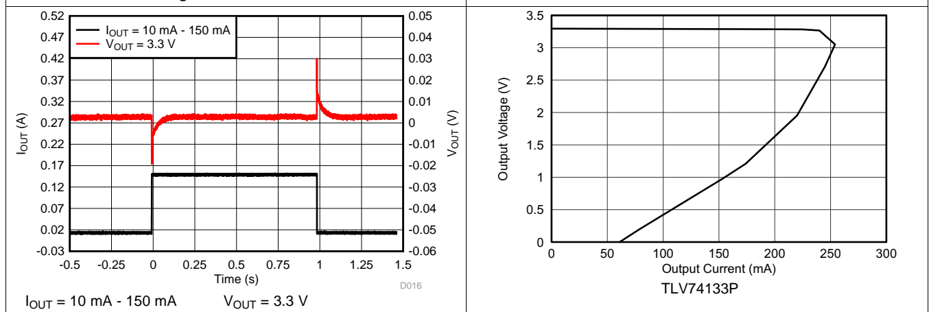
Figure 17. Load Transient
