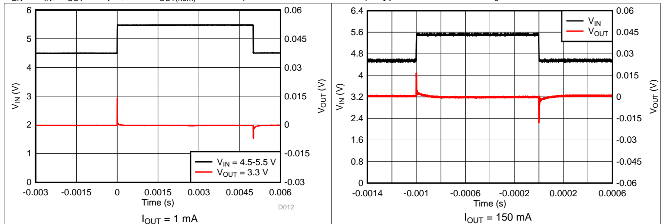
Figure 13. Line Transient
