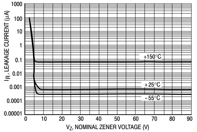
Figure 7. Typical Leakage Current
