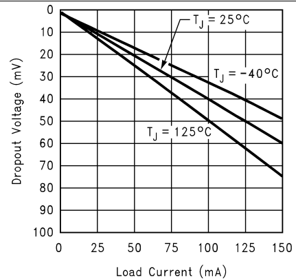
Figure 4. Dropout Voltage vs Load Current
