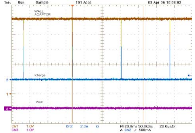
Figure 14. Output Short Circuit
