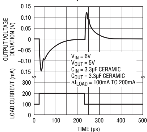
Transient Response
