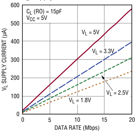
V_L Supply Current vs Data Rate
