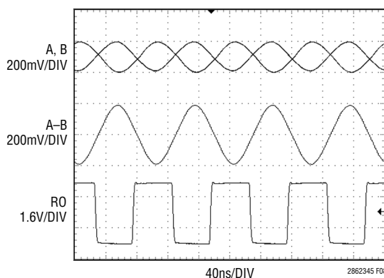
Figure 8. Duty Cycle of Balanced Receiver with \pm 200mV 10Mbps Input Signal
