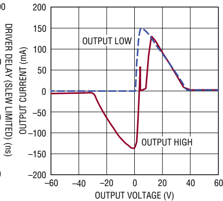
Driver Output Short-Circuit Current vs Voltage
