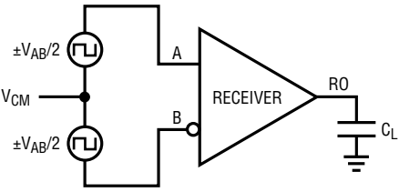
Figure 6. Receiver Propagation Delay Measurements
