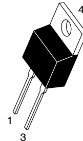
TO-220AC CASE 221B STYLE 2
