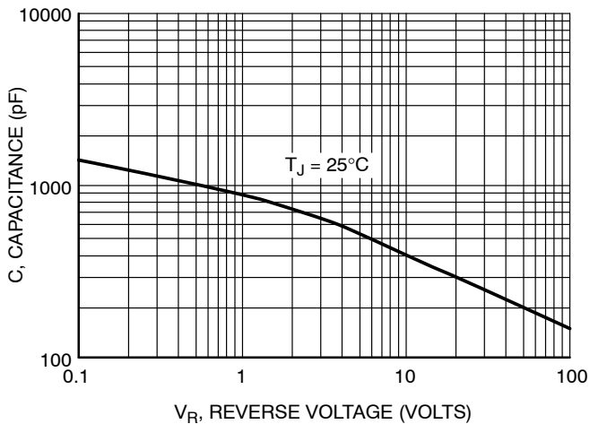
Figure 7. Maximum Capacitance
