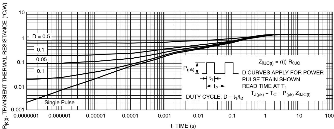
Figure 9. Thermal Response
