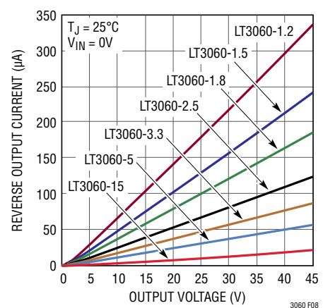
Figure 8. LT3060-1.2/-1.5/-1.8/-2.5/-3.3/-5/-15 Reverse Output Current
