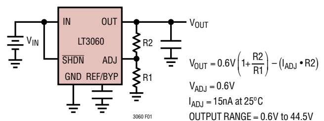
Figure 1. Adjustable Operation
