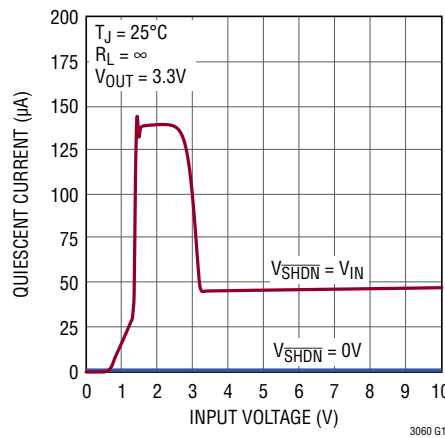
LT3060-3.3 Quiescent Current
