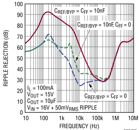
LT3060-15 Input Ripple Rejection
