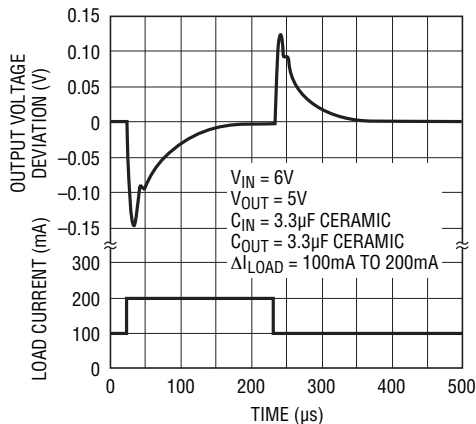
Transient Response
