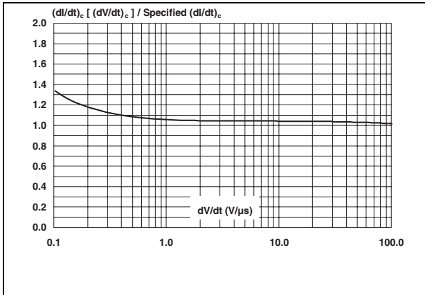
Figure 9. Relative variation of critical rate of decrease of main current (di/dt) c versus reapplied (dV/dt) c
