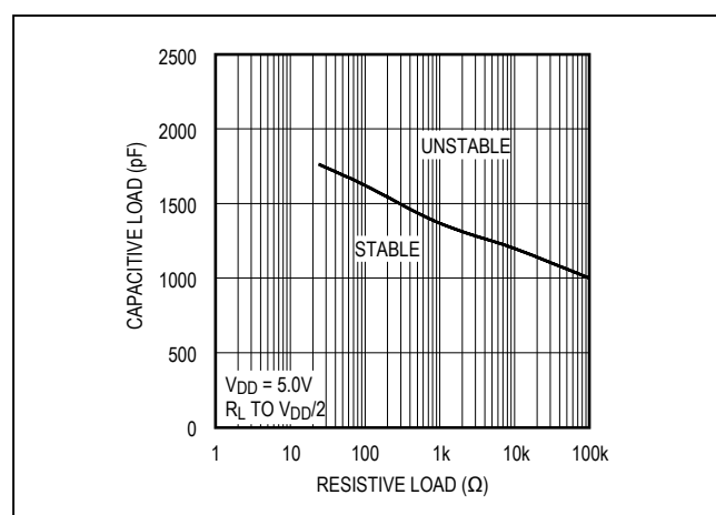
Figure 6. Capacitive-Load Stability
