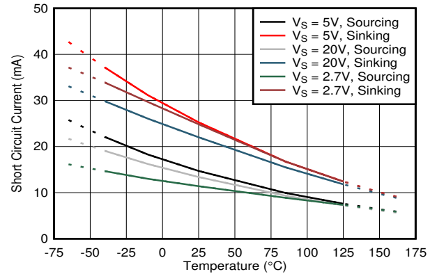
Figure 5-20. Short-Circuit Current vs Temperature
