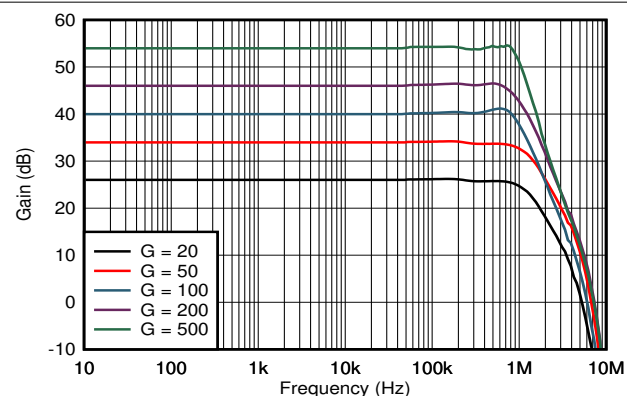
Figure 5-3. Gain vs Frequency
