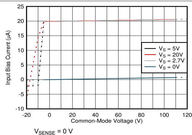
Figure 5-5. Input Bias Current vs Common-Mode Voltage
