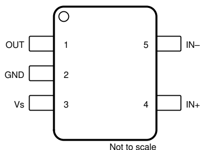
Figure 4-2. INA281B: DBV Package 5-Pin SOT-23 Top View
