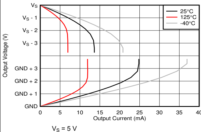
Figure 5-11. Output Voltage vs Output Current
