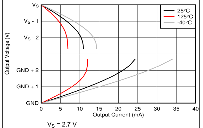
Figure 5-10. Output Voltage vs Output Current
