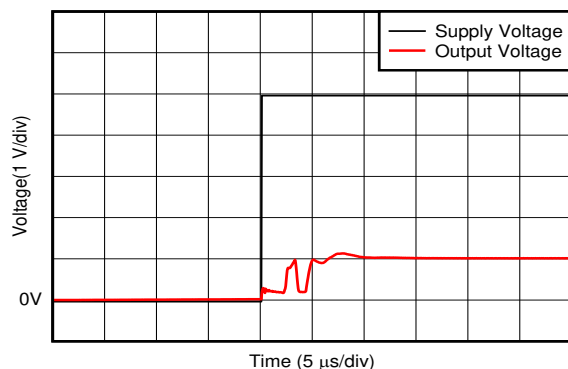
Figure 5-25. Start-Up Response
