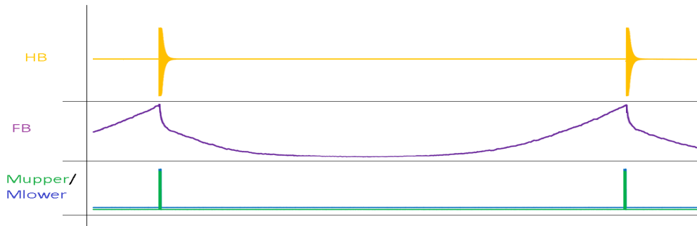
Figure 18. No-load Operation
