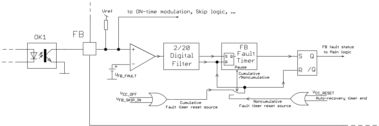
Figure 10. Internal FB Fault Management
