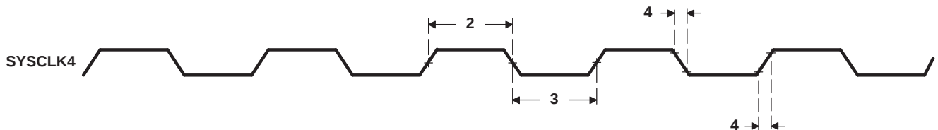
Figure 7-22. SYSCLK4 Timing
