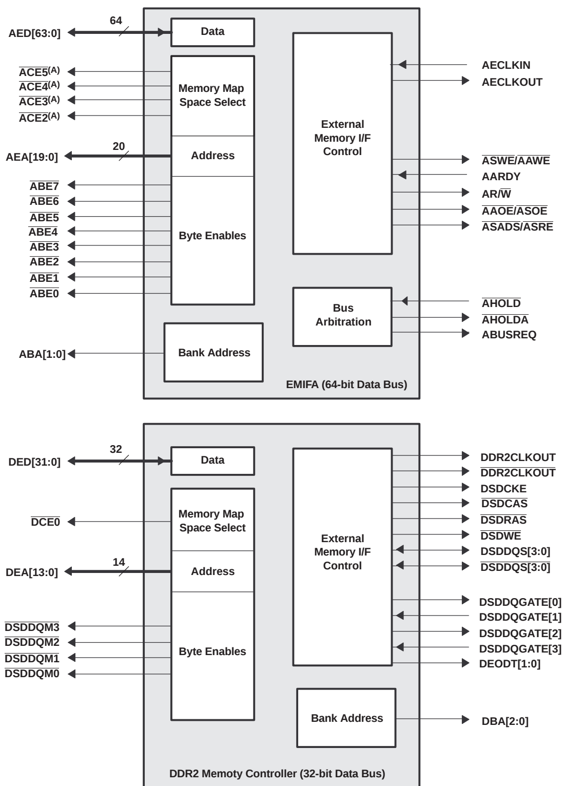
Figure 2-8. EMIFA and DDR2 Memory Controller Peripheral Signals
