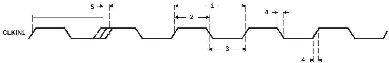
Figure 7-21. CLKIN1 Timing
