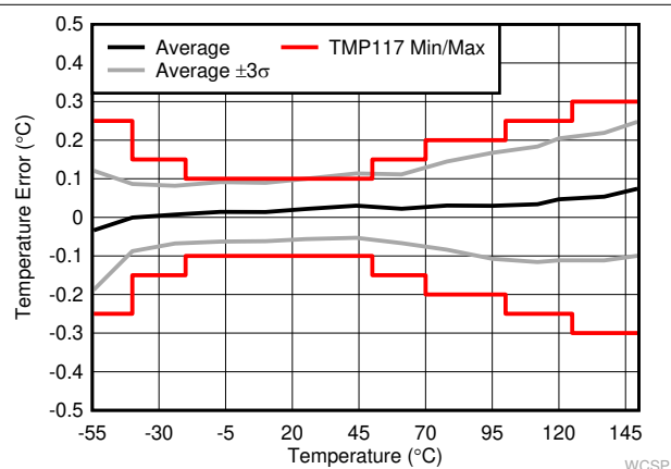
Figure 6-3. YBG Package Temperature Error vs Temperature
