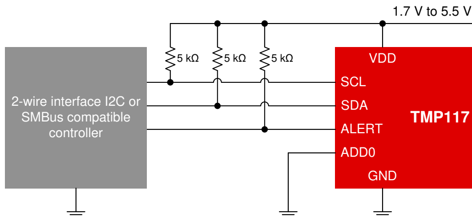
Figure 8-1. Typical Connections
