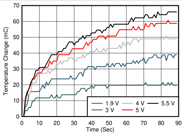
Figure 8-2. Self-Heating in Still Air vs. Temperature and Dissipated Power
