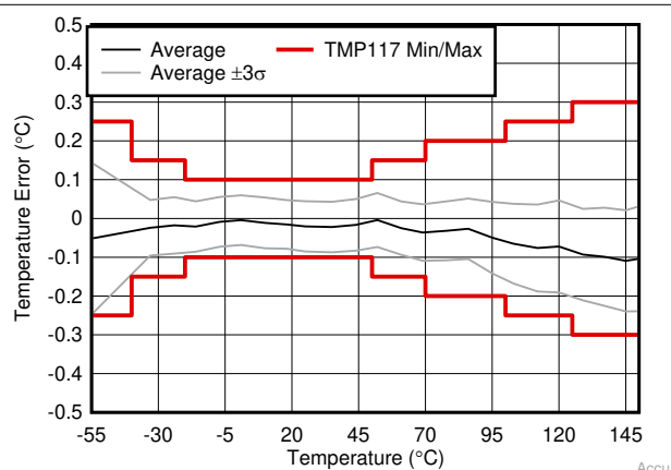
Figure 6-2. DRV Package Temperature Error vs Temperature
